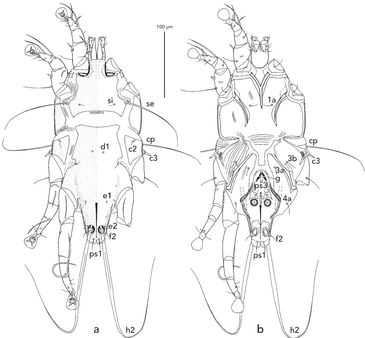
Fig. 1 Alloptes ( Conuralloptes ) aechemorhynchi , male: a, dorsal view; b, ventral view.
