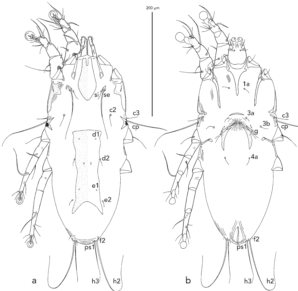
Fig. 6 Ingrassia platyspina , female: a, dorsal view; b, ventral view.
