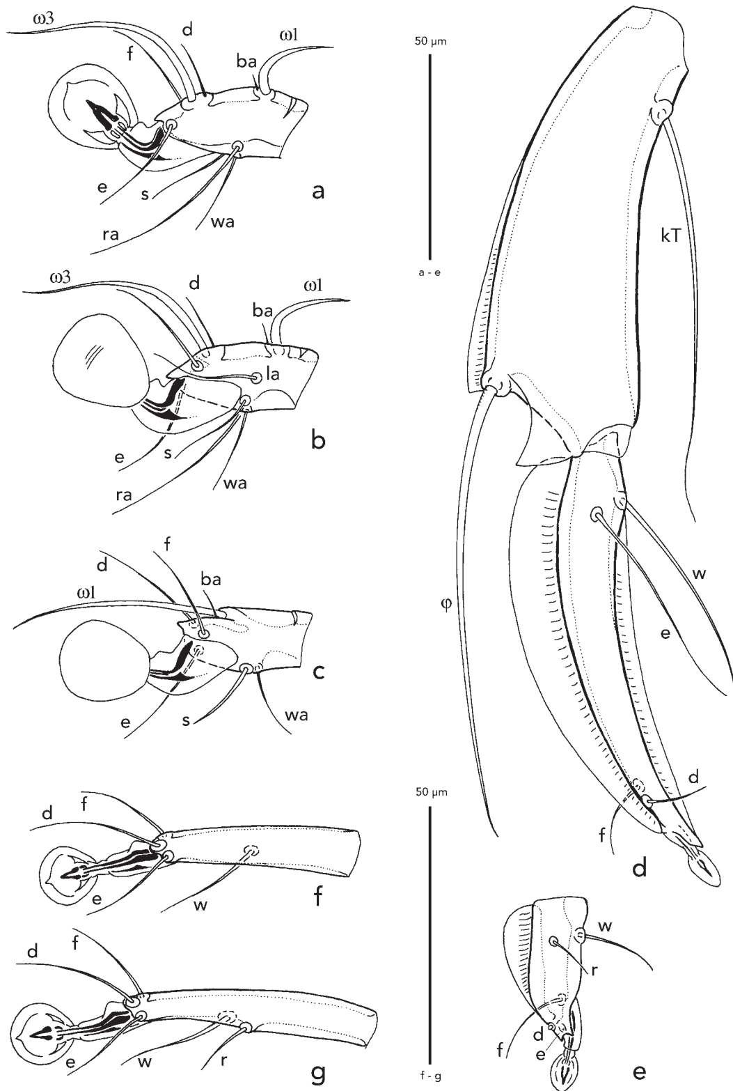
Fig. 5 Ingrassia platyspina , a–e, male; f–g, female: a, tarsus I, dorsal view; b, tarsus I, ventral view; c, tarsus II, ventral view; d, tibia and tarsus III, dorsal view; e, tarsus IV, dorsal view; f, tarsus III, dorsal view; g, tarsus IV, dorsal view.
