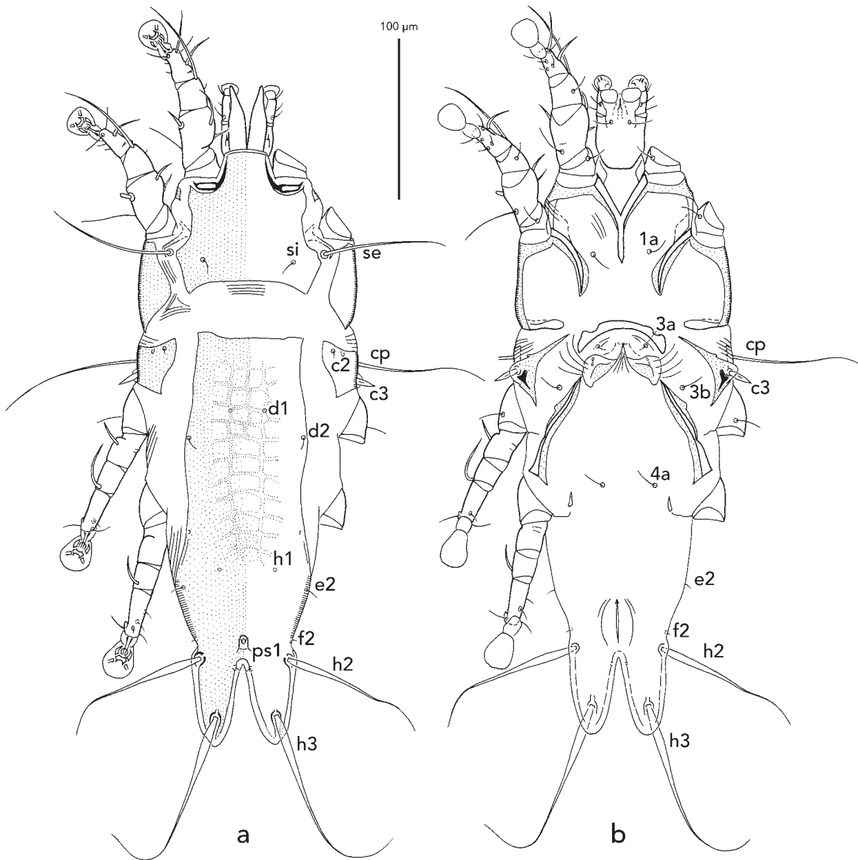
Fig. 3 Alloptes (Conuralloptes) aechmorhynchi , female: a, dorsal view; b, ventral view.
